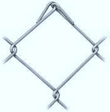
Selvage: Knuckle
